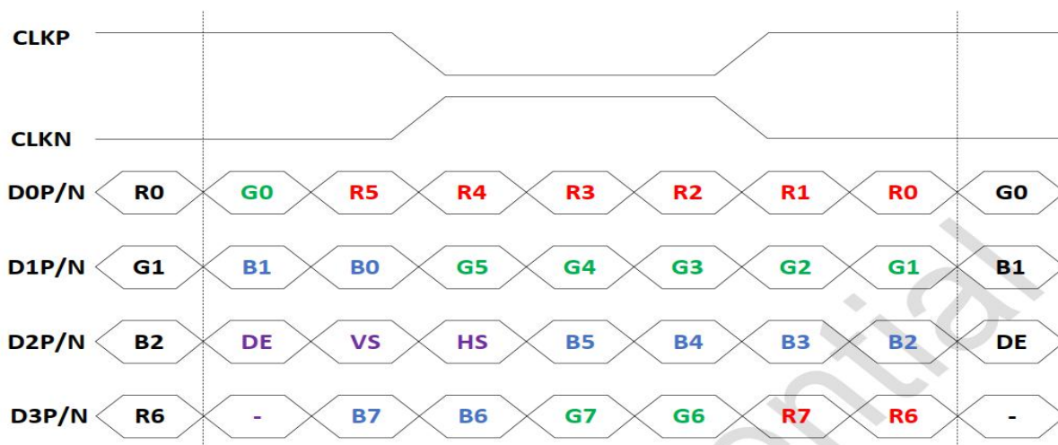
8-bit LVDS Interface data format
